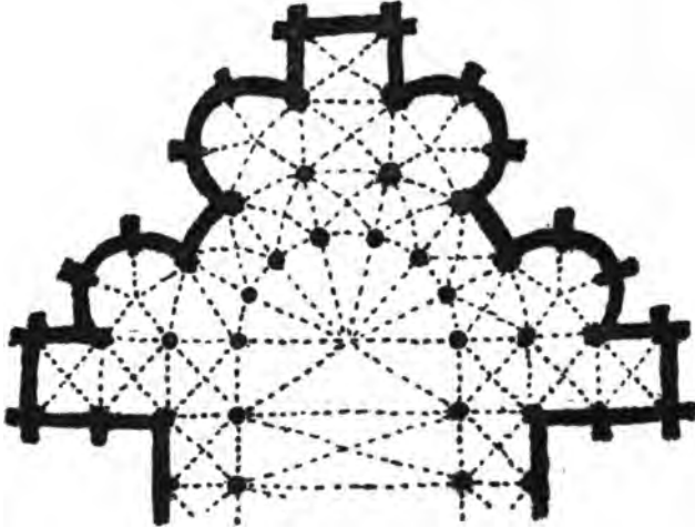
FIG. 72. Destroyed abbey church of Vaucelles, near Cambrai.
